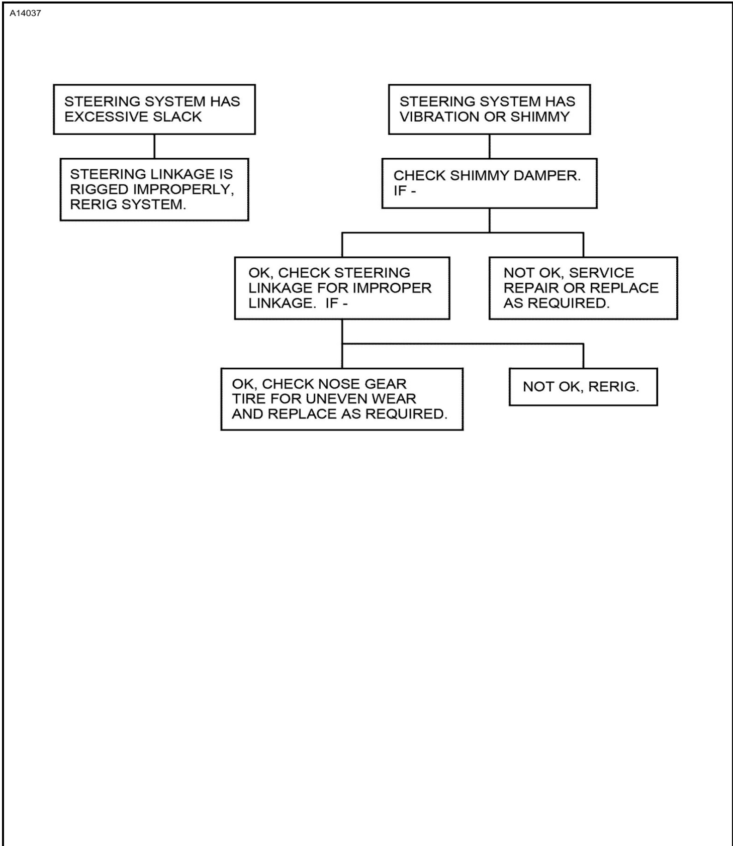
Figure 101 : Sheet 2 : Nose Gear Steering
